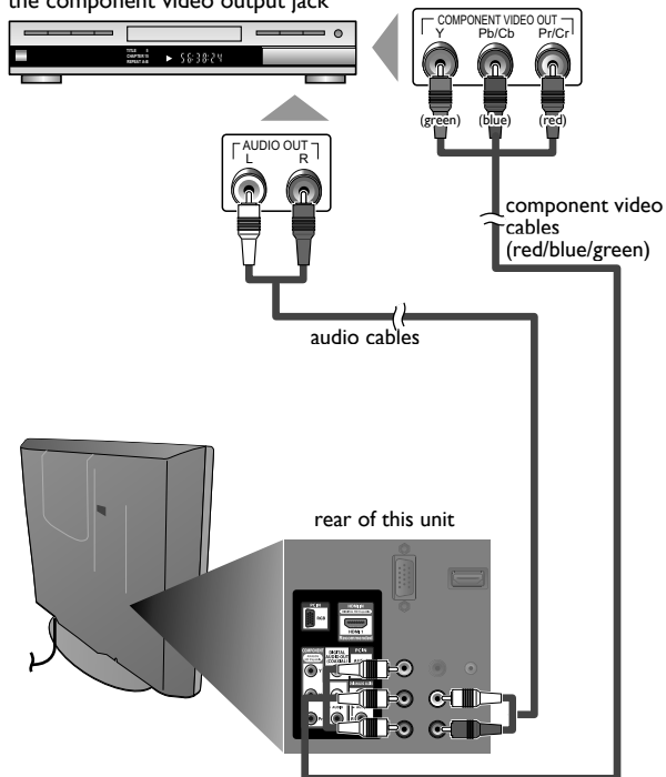
BD/DVD recorder with the component video output jack
